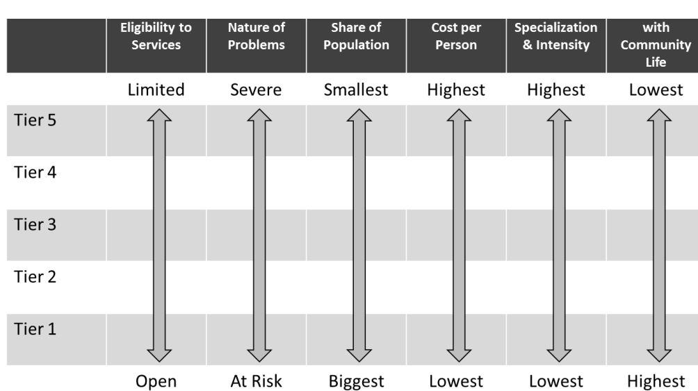
Figure 3: Criteria for Defining Tiered Substance Use Treatment Responses (adapted from Rush, 2010)
